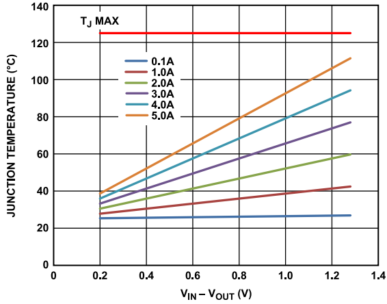
Figure 51. 500 mm 2 of PCB Copper, T_B = 25^\circ\text{C}
