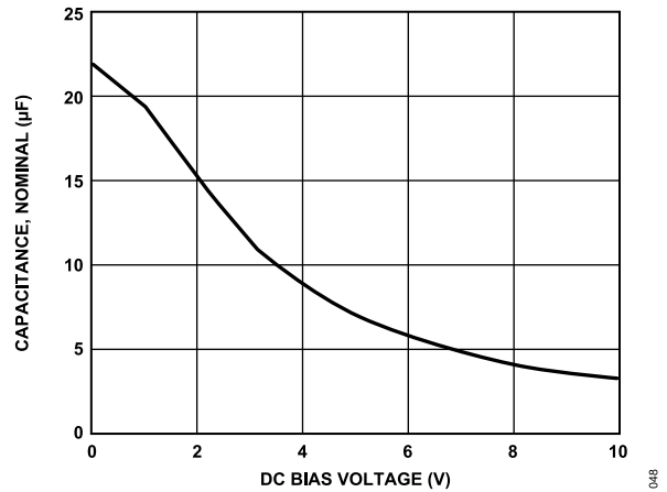
Figure 48. Capacitance vs. DC Bias Voltage
