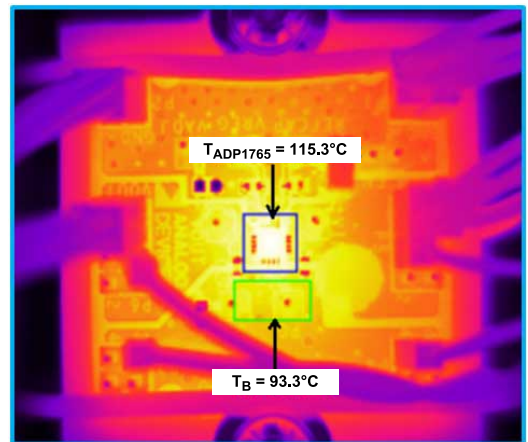
Figure 56. Thermal Image of the ADP1765 Evaluation Board at I_{LOAD} = 5\text{A} , V_{IN} = 1.5\text{V} , V_{OUT} = 1.3\text{V} , T_B = 93.3^\circ\text{C}
