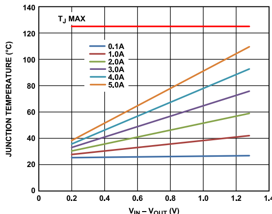
Figure 50. 1000 mm 2 of PCB Copper, T_B = 25^\circ\text{C}
