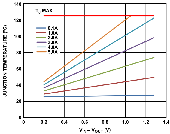
Figure 52. 100 mm 2 of PCB Copper, T_B = 25^\circ\text{C}
