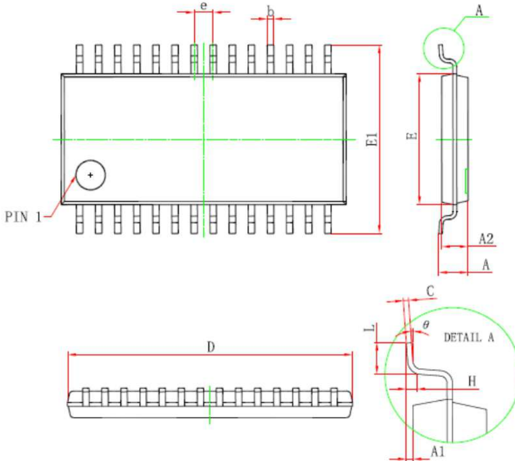
TSSOP28 PACKAGE OUTLINE DIMENSIONS
