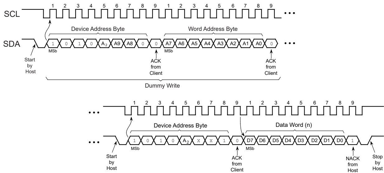
Figure 8-2. Random Read
