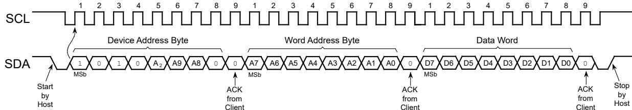
Figure 7-1. Byte Write
