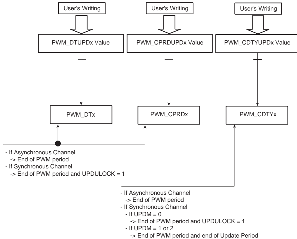
Figure 50-34. Synchronized Period, Duty-Cycle and Dead-Time Update
