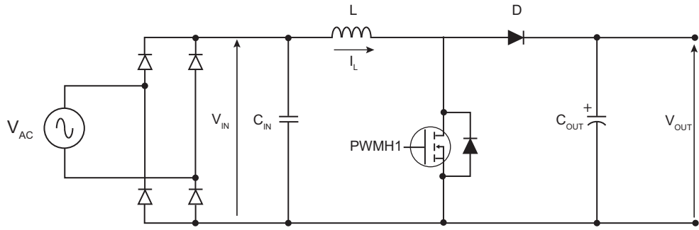
Figure 50-28. External PWM Reset Mode: Power Factor Correction Application
