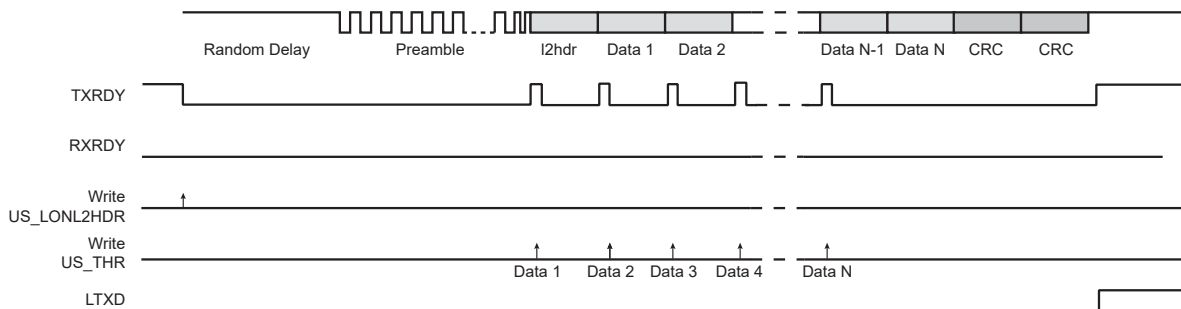
Figure 45-61. Tx Frame
