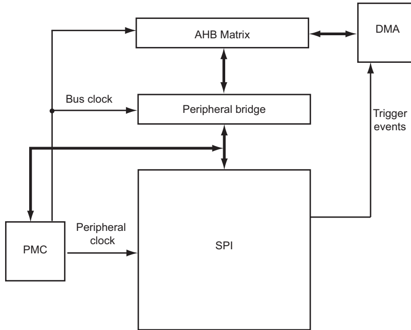
Figure 40-1. Block Diagram
