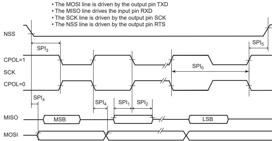
Figure 57-27. USART SPI Client Mode (Mode 1 or 2)
