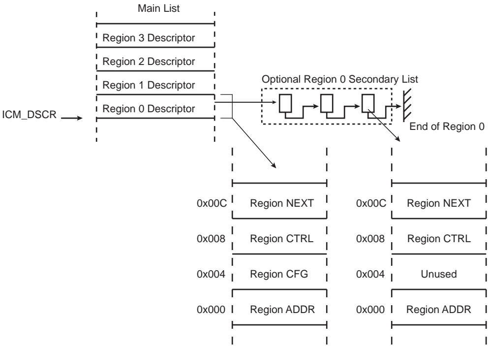
Figure 54-4. Region Descriptor
