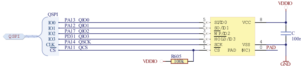
Figure 59-5. Schematic Example with QSPI Data Flash
