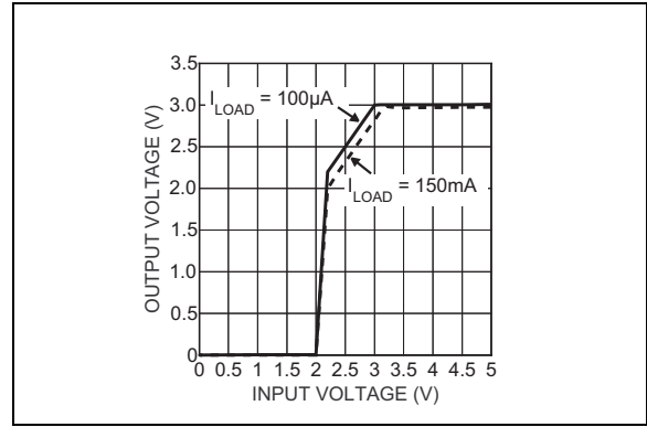
FIGURE 2-11: Dropout Characteristics.
