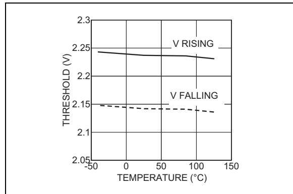
FIGURE 2-24: UVLO Threshold vs. Temperature.
