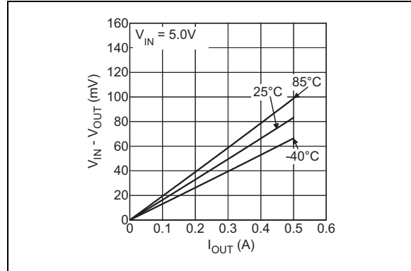
FIGURE 2-22: V_{DROP} vs. Temperature (MIC20XXA).
