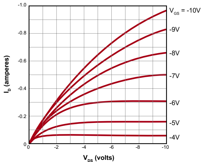
Saturation Characteristics
