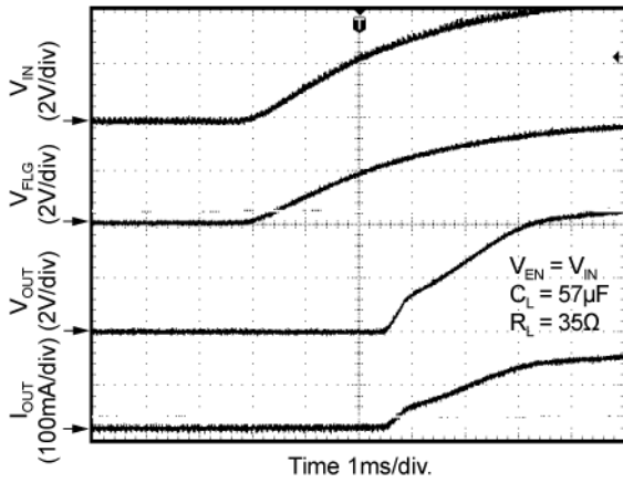
Turn-On/Turn-Off (MIC2026A-1)
