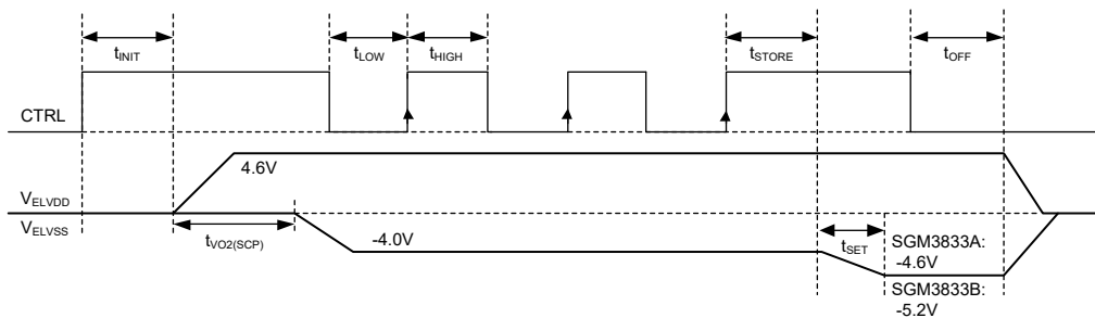
Figure 2. Timing Diagram
