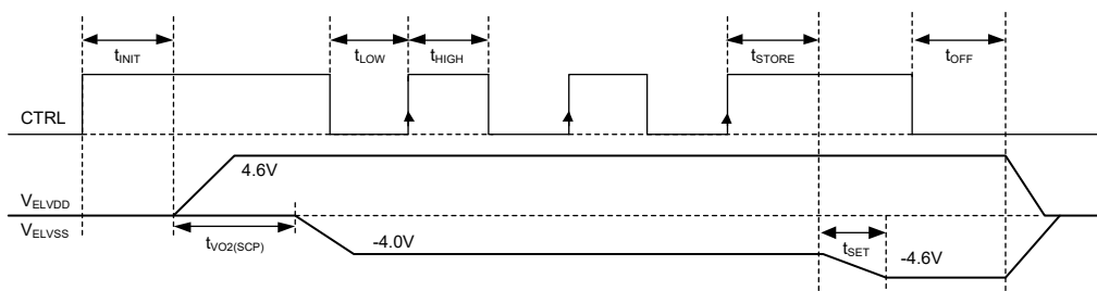
Figure 3. SGM3833A Programming V ELSS
