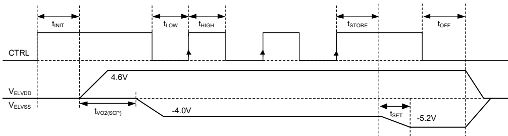
Figure 4. SGM3833B Programming V ELSS
