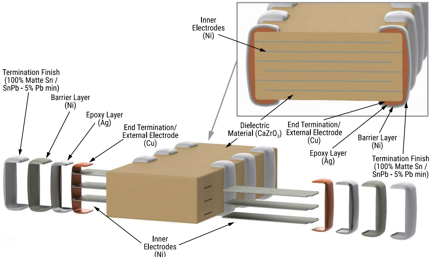
Detailed Cross Section
