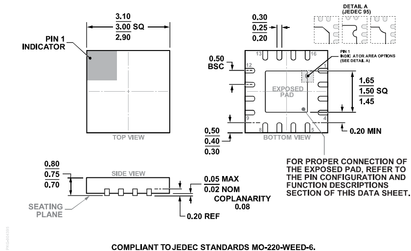
Figure 26. 16-Lead Lead Frame Chip Scale Package [LFCSP] 3 mm x 3 mm Body and 0.75 mm Package Height (CP-16-27)
