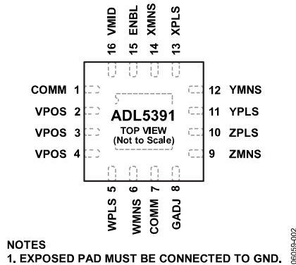
Figure 2. Pin Configuration
