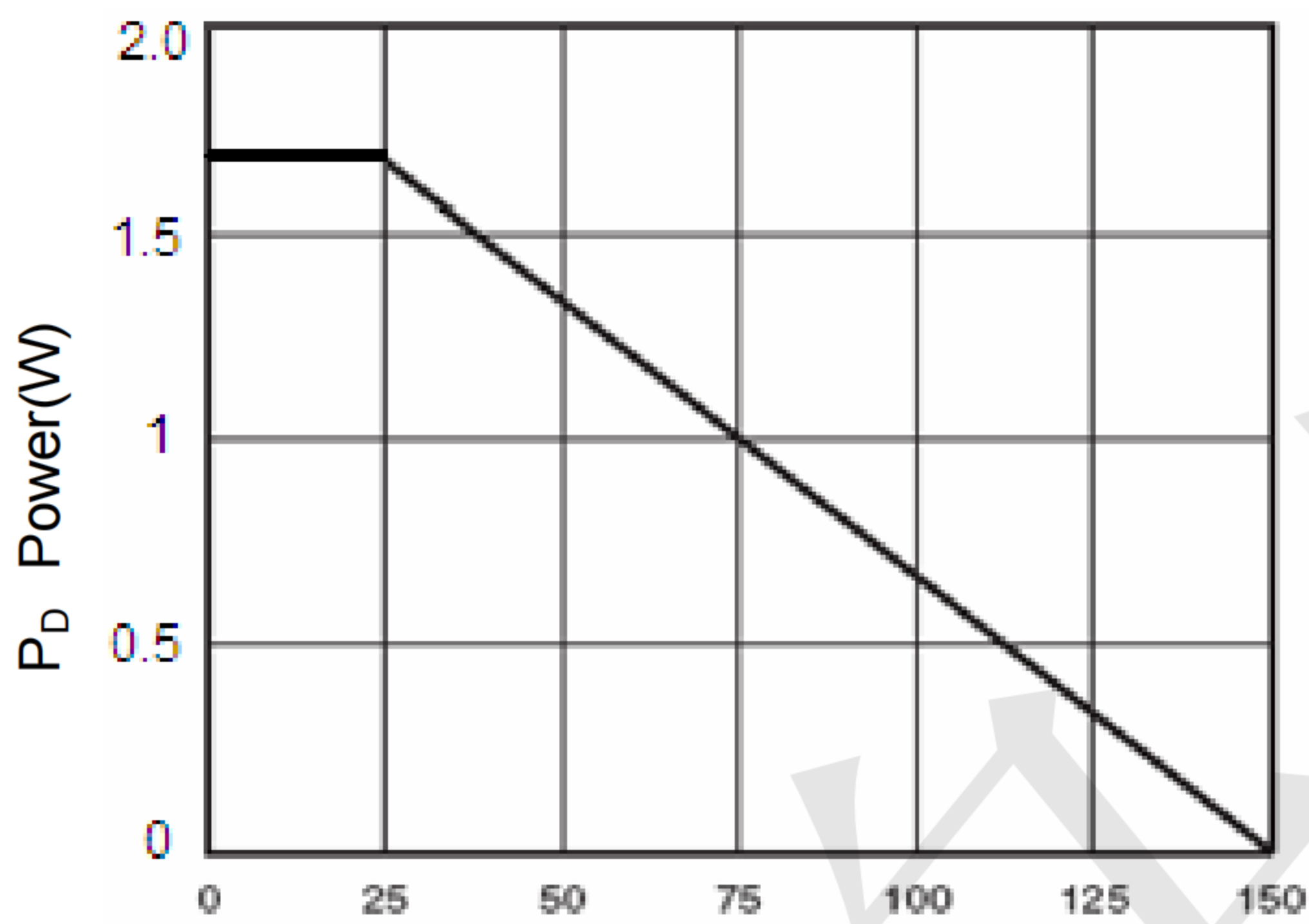
Figure 3 Power Dissipation
