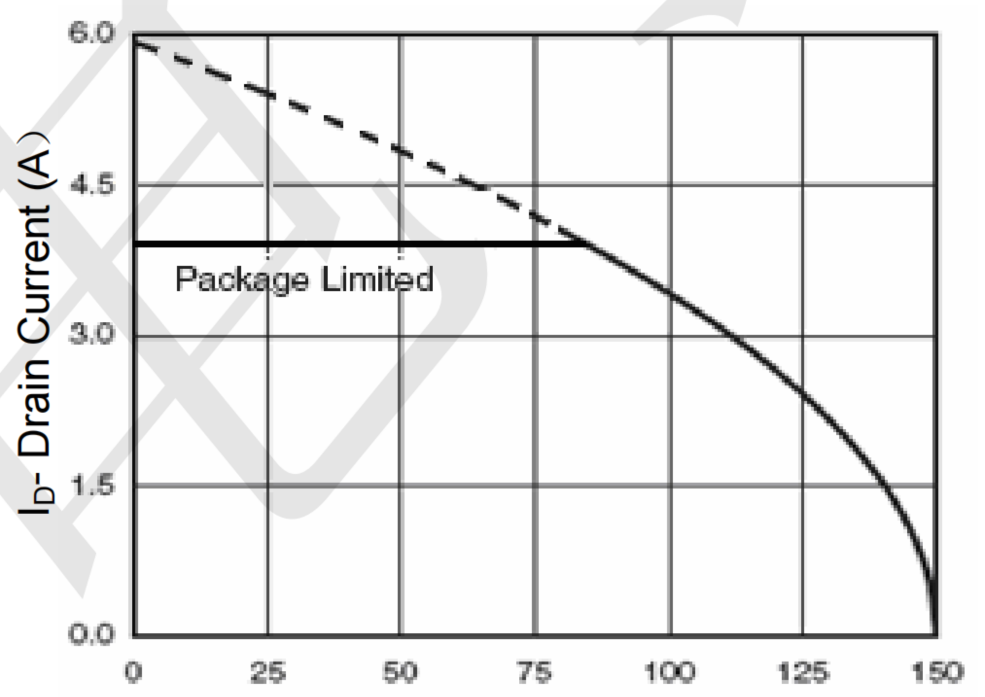
Figure 4 Drain Current
