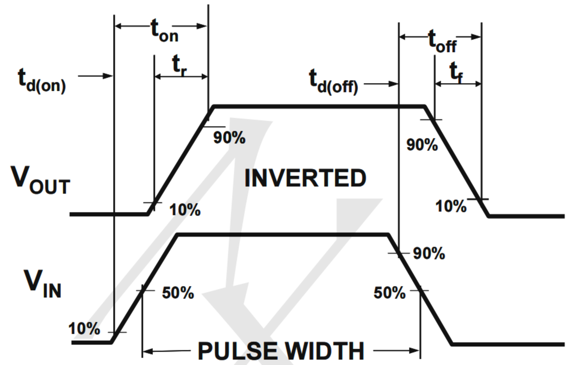
Figure 2: Switching Waveforms
