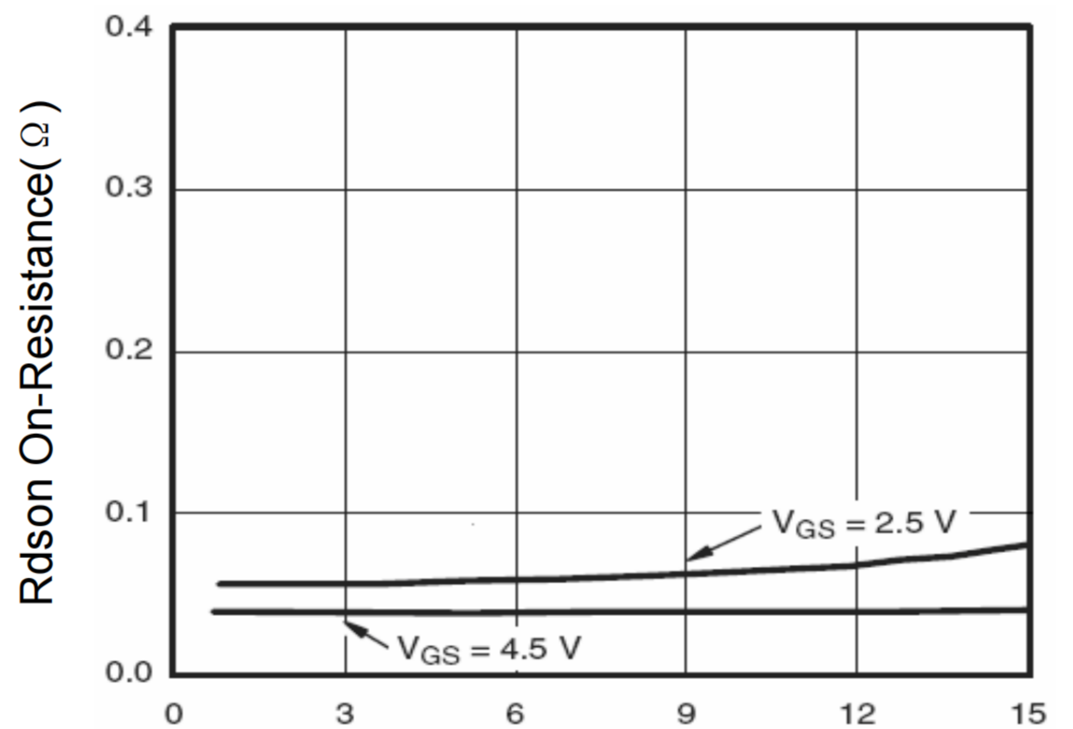
Figure 6 Drain-Source On-Resistance
