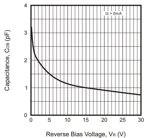
Fig.4 - Output Capacitance
