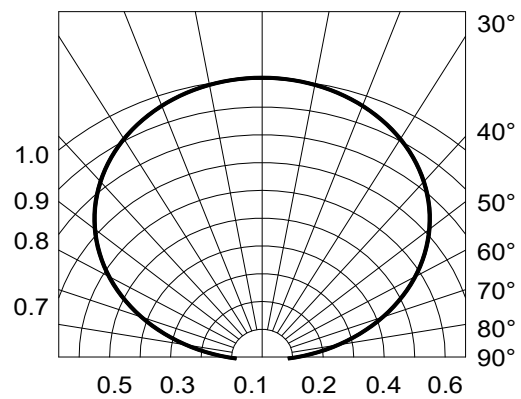
Fig.6-Radiation Diagram Ta=25°C 0° 10° 20°
