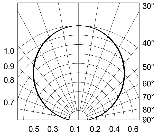
Fig.6-Radiation Diagram T_a=25^\circ\text{C}
