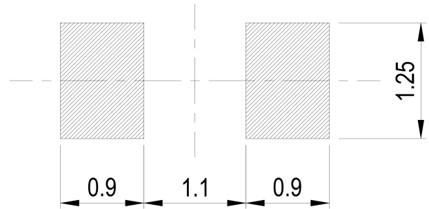
Recommended Solder Pad
