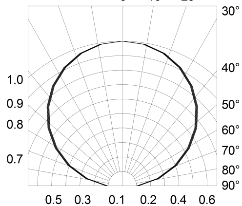
Fig.6-Radiation Diagram Ta=25°C
