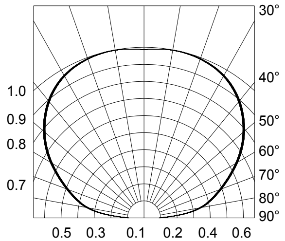
Fig.6-Radiation Diagram Ta=25°C
