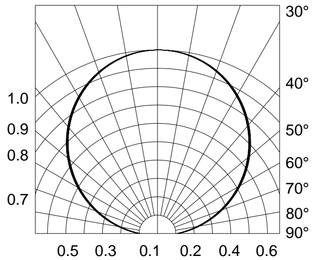
Fig.6-Radiation Diagram Ta=25°C
