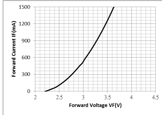
Fig 4. Forward Current
