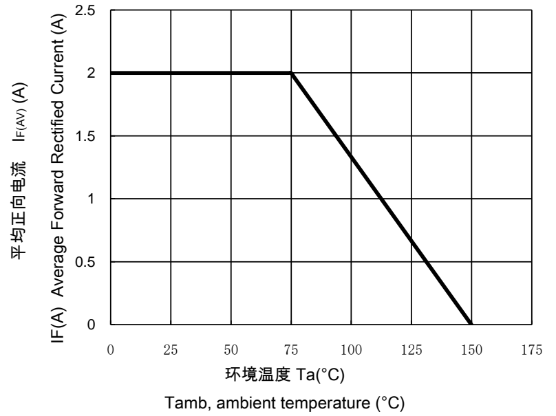
FORWARD CURRENT DERATING CURVE
