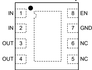
TDFN-3x3-8L
