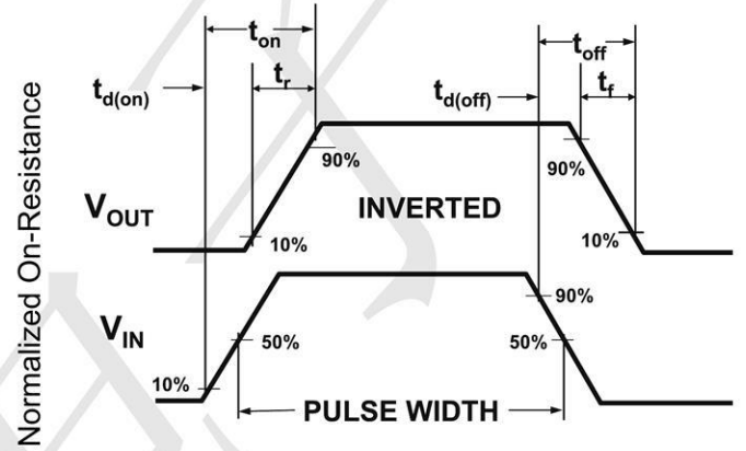
Figure 2: Switching Waveforms
