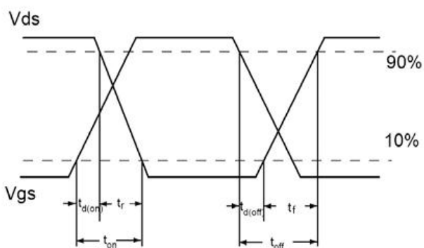
Switch Waveforms:
