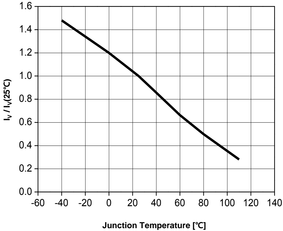
Fig 6. Relative Light Output vs. Junction Temperature, I_F = 140\text{mA}
