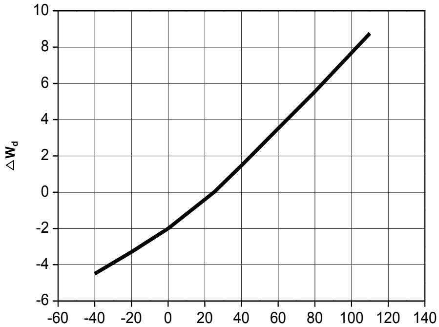
Fig 8. Dominant wavelength shift vs. Junction Temperature, I_F = 140\text{mA}
