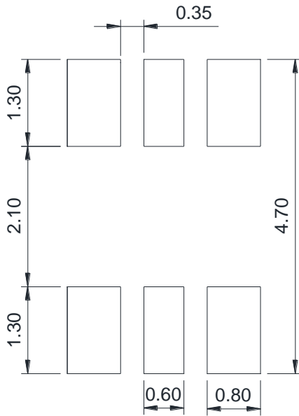
<Recommended solder pad>
