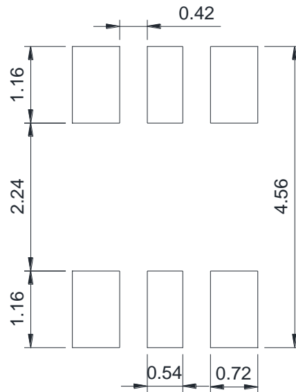
<Recommended stencil pattern>
