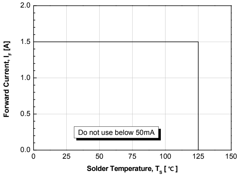
Fig 9. Solder Temperature vs. Allowable Forward Current
