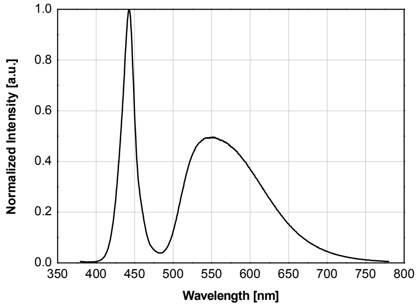
Fig 1. Color Spectrum, I_F = 1.0A , T_a = 25^\circ C
