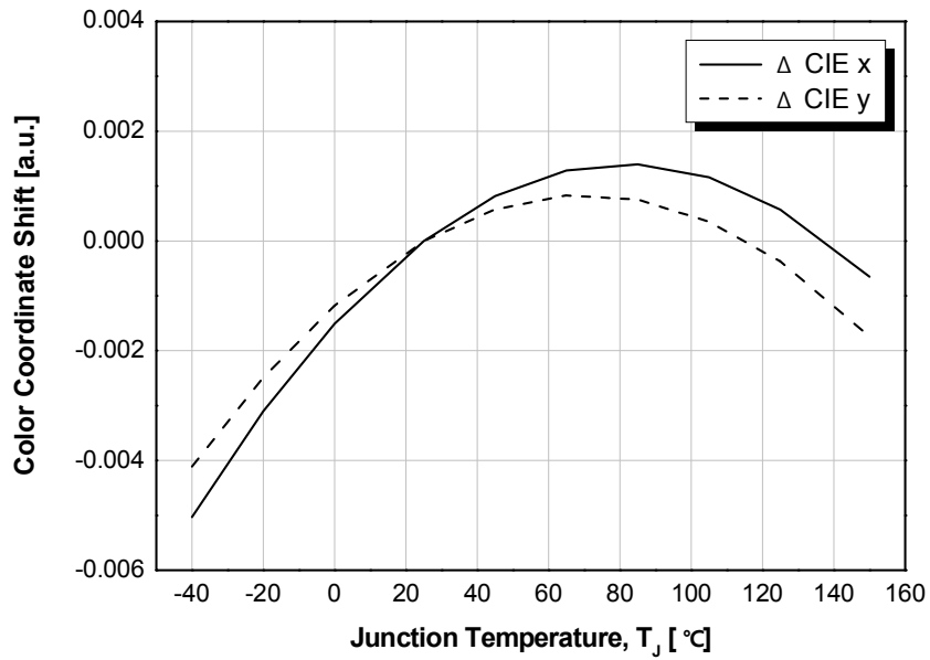
Fig 8. Junction Temperature vs. Color Coordinate Shift, I_F = 1.0A
