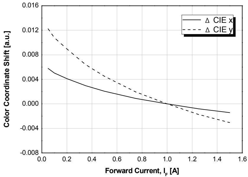
Fig 5. Forward Current vs. Color Coordinate Shift, T_a = 25^\circ\text{C}
