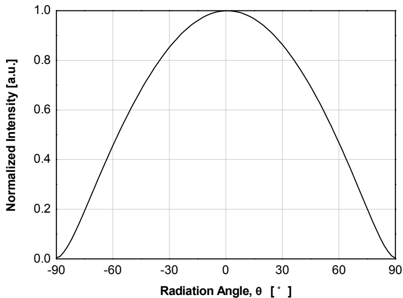
Fig 2. Radiant Pattern, T_a = 25^\circ C
