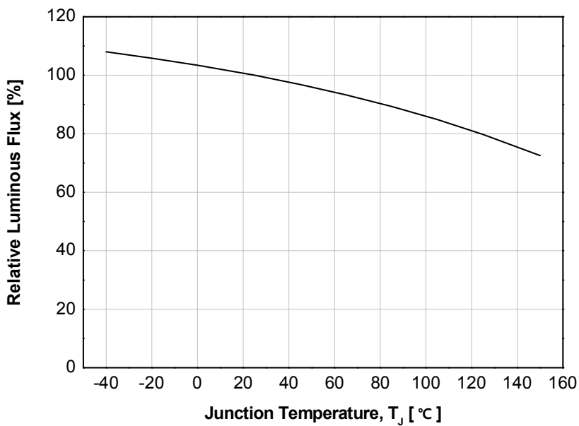
Fig 7. Junction Temperature vs. Relative Luminous Flux, I_F = 1.0A
