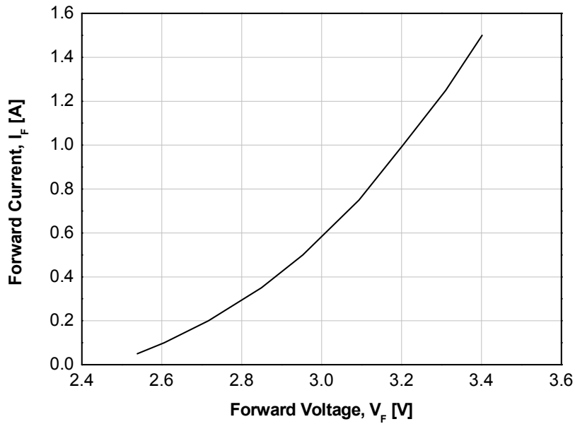
Fig 3. Forward Voltage vs. Forward Current, T_a = 25^\circ\text{C}
