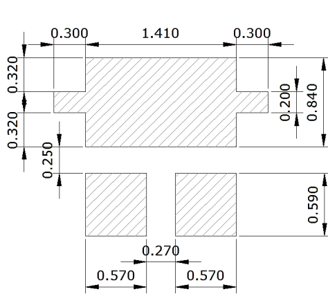
Solder Pad
