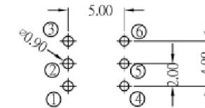
P.C.B.LAYOUT(TOP VIEW)
