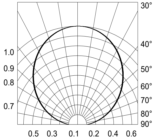
Fig.6-Radiation Diagram Ta=25°C
