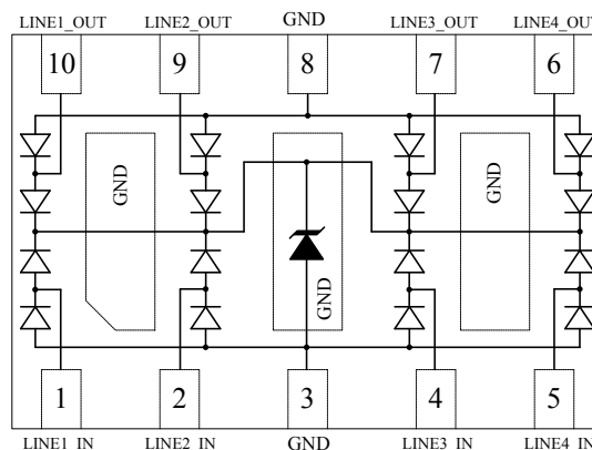
DFN3.0×2.0-10L (Top View)
