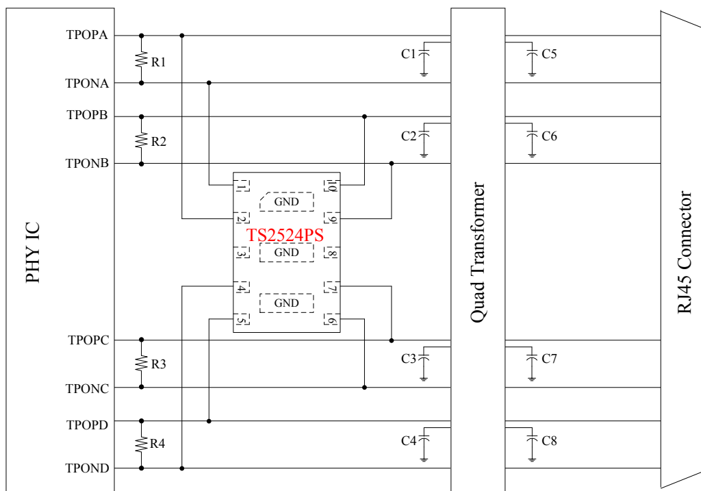
Schematic Diagram for Gigabit Ethernet ESD/Surge Protection using TS2524PS
