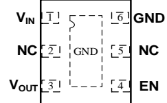
DFN(2*2)-6 Top View
