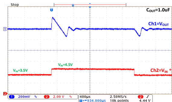
Line Transient: MD5125F ( I_{OUT}=1mA )
