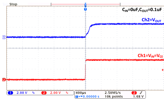
Power Up: MD5125F ( I_{OUT}=1mA )
