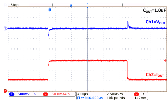
Load Transient: MD5125F ( I_{OUT}=50mA\sim 100mA\sim 50mA )
