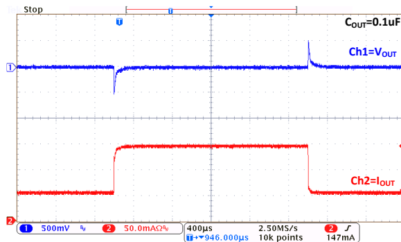
Load Transient: MD5125F ( I_{OUT}=50mA\sim 100mA\sim 50mA )
