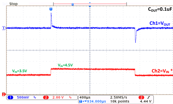
Line Transient: MD5125F ( I_{OUT}=10mA )
