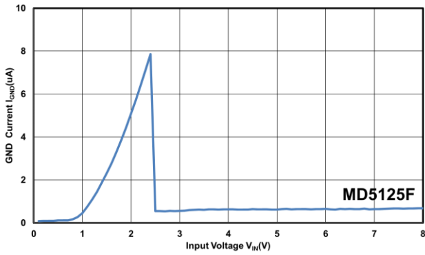
GND Current vs. Input Voltage ( C_{OUT}=0.1\mu F )
