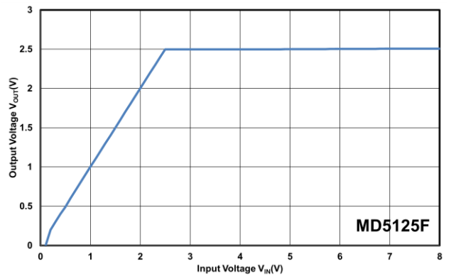
Output Voltage vs Input Voltage ( C_{OUT}=0.1\mu F )
