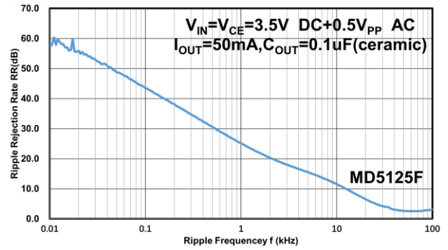
MD5125F Power Supply Rejection Ratio
