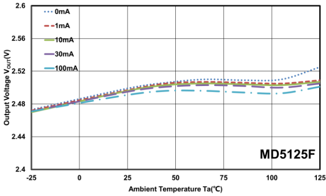
Output Voltage vs. Temperature ( C_{OUT}=0.1\mu F )
