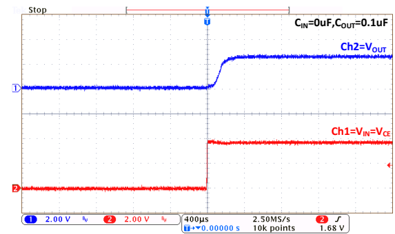
Power Up: MD5125F ( I_{OUT}=100mA )
