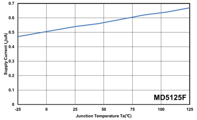
Supply Current vs. Temperature ( C_{OUT}=0.1\mu F )
