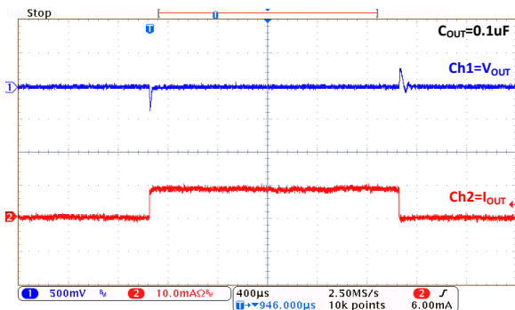
Load Transient: MD5125F ( I_{OUT}=1mA\sim 10mA\sim 1mA )
