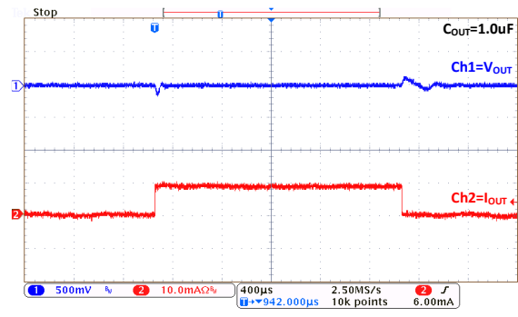
Load Transient: MD5125F ( I_{OUT}=1mA\sim 10mA\sim 1mA )
