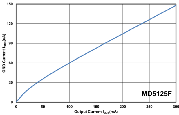
GND Current vs Output Current ( C_{OUT}=1.0\mu F )
