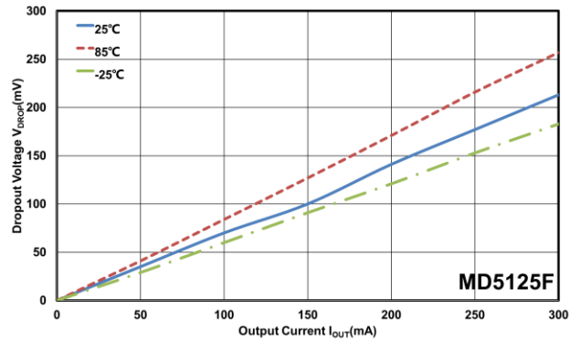
Dropout Voltage vs. Output Current ( C_{OUT}=0.1\mu F )
