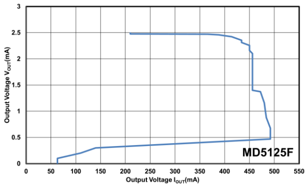
MD5125F Output Current Fold-back
