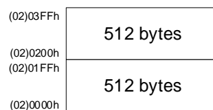
SC95FS52X 1 Kbytes LDROM Sector 示意
