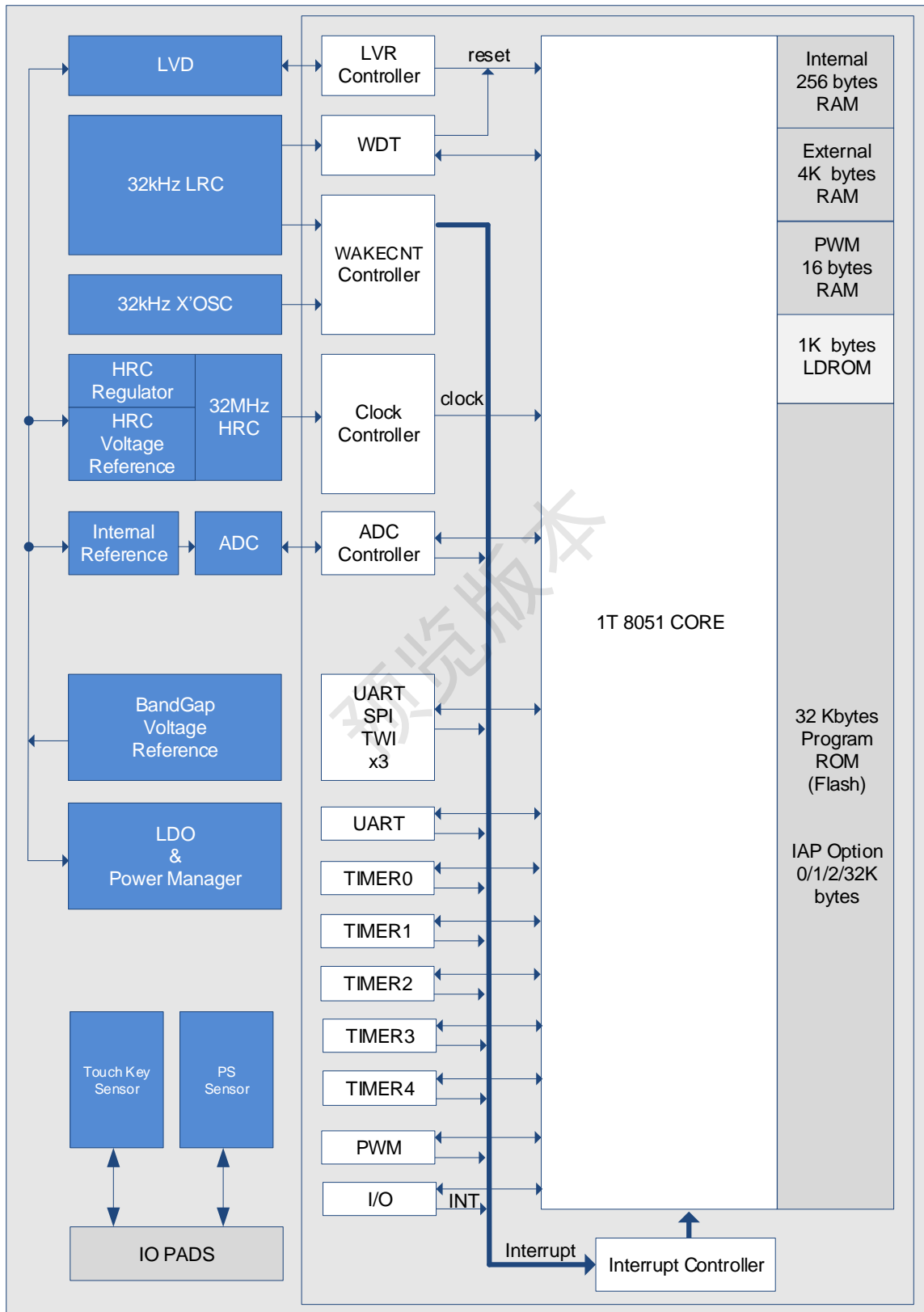
SC95FS52X BLOCK DIAGRAM
