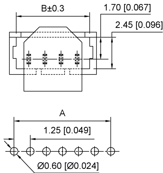
Recommended PCB Layout(Top view) Tolerance:±0.05mm
