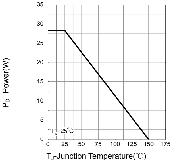
Figure 3 Power Dissipation
