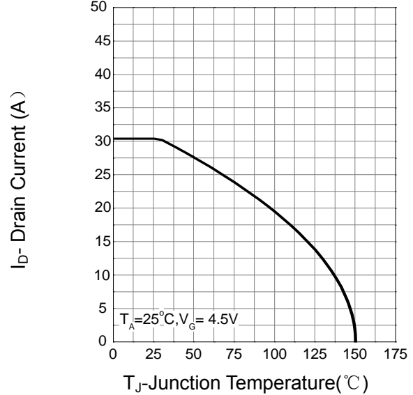
Figure 4 Drain Current
