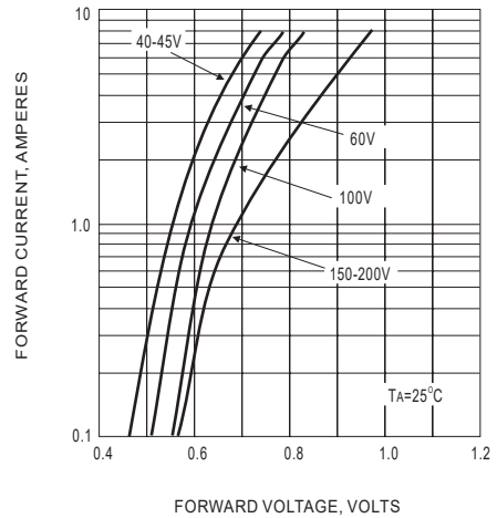
FIG.2-TYPICAL FORWARD CHARACTERISTICS
