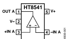
Figure 1. 5-Lead SC70 and 5-Lead SOT-23 (KS and R Suffixes)
