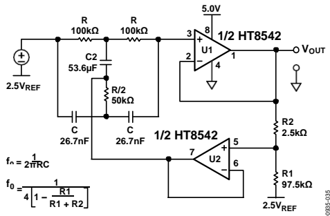
Figure 35. 60 Hz Twin-T Notch Filter, Q = 10
