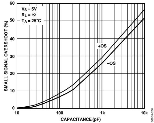
Figure 26. Small Signal Overshoot vs. Load Capacitance
