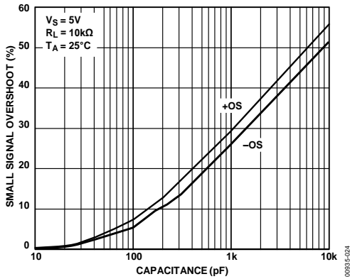
Figure 24. Small Signal Overshoot vs. Load Capacitance
