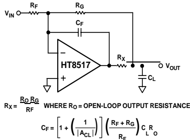
Figure 22. In-the-Loop Compensation Technique for Driving Capacitive Loads
