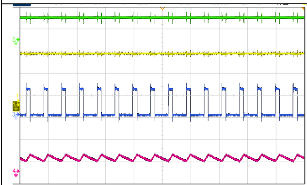
Fig.13 Steady State, Iout =5A
