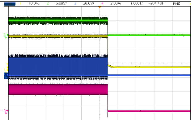
Fig.10 Shut down waveform, Iout =5A
