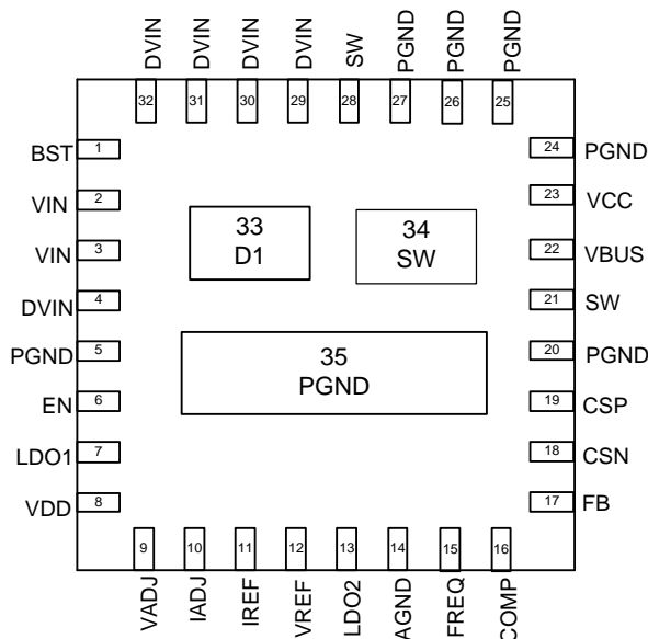
Fig. 2 Pin-Function (QFN5X5-32)
