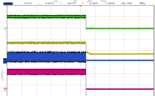
Fig.8 Shut down waveform, Iout =5A
