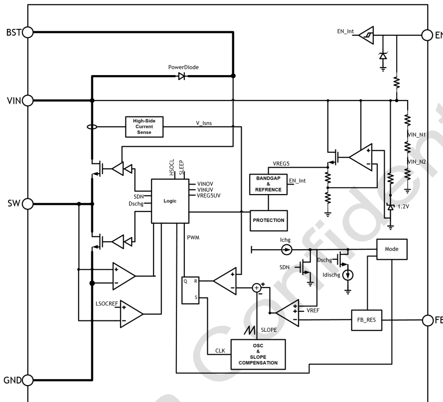
Fig.22 PL88104 Diagram
