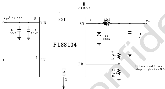
Fig 24 Schematic
