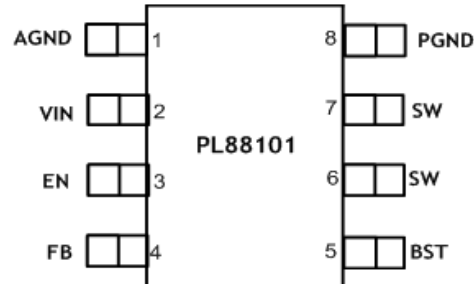
Fig.4 SOP8 Package
