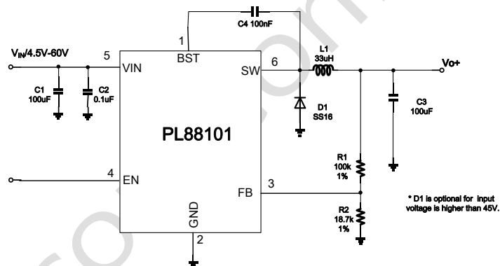
Fig. 1 Schematic (SOT23-6L Package)
