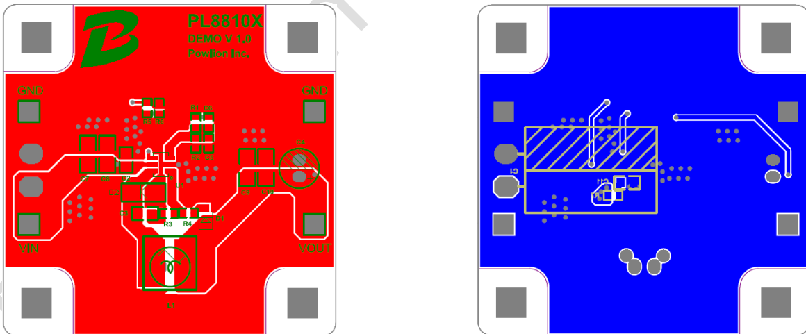
Fig 25 PCBLayout
