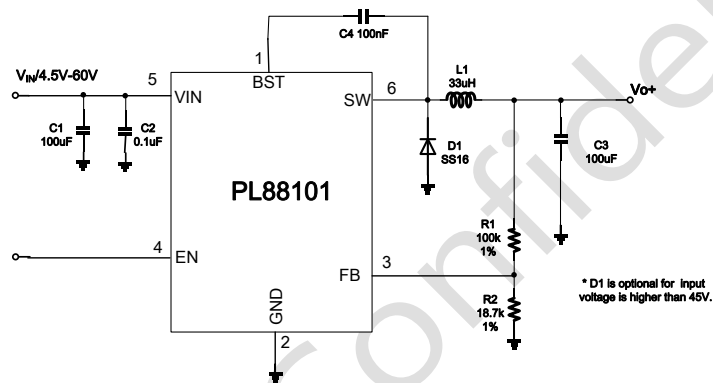
Fig 24 Schematic
