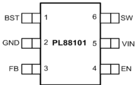
Fig.3 SOT23-6L Package
