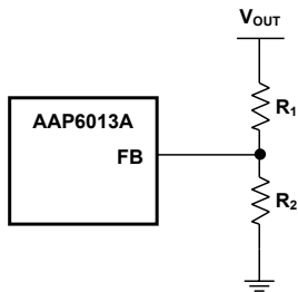
Figure 3. Setting V_{OUT} with an External Resistor Divider
