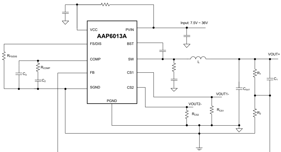
Figure 1. Simplified Schematic
