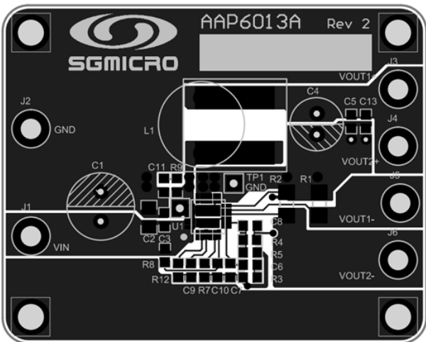
Figure 5. PCB Top Layer
