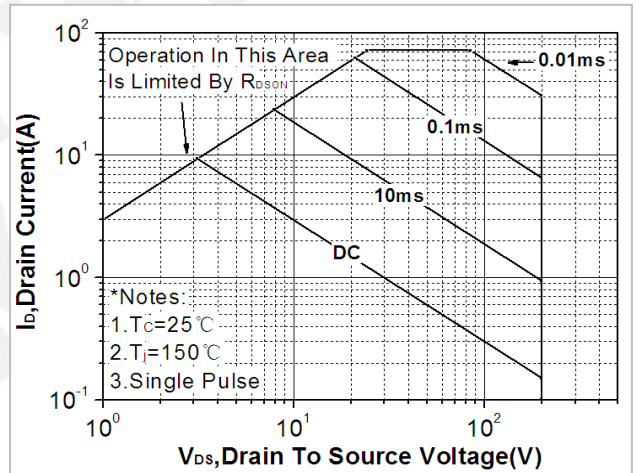
Fig. 10. Maximum safe operating area(TO-220FT)
