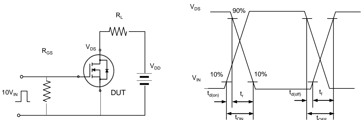
Fig. 18. Switching time test circuit & waveform
