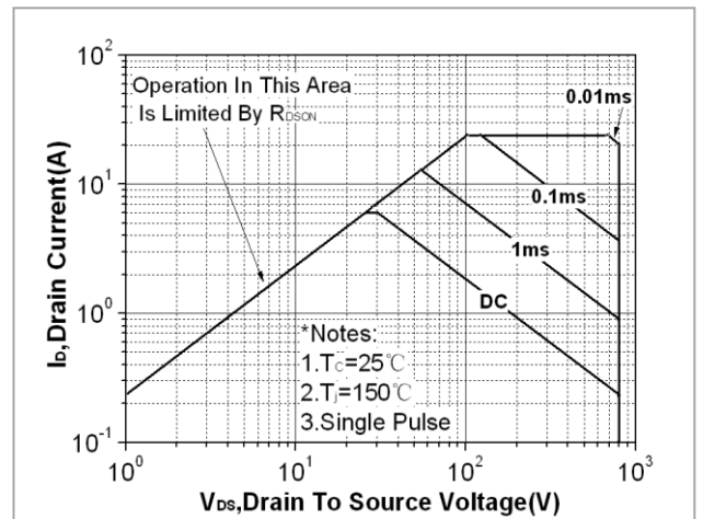
Fig. 12. Maximum safe operating area (TO-262&TO-262N)
