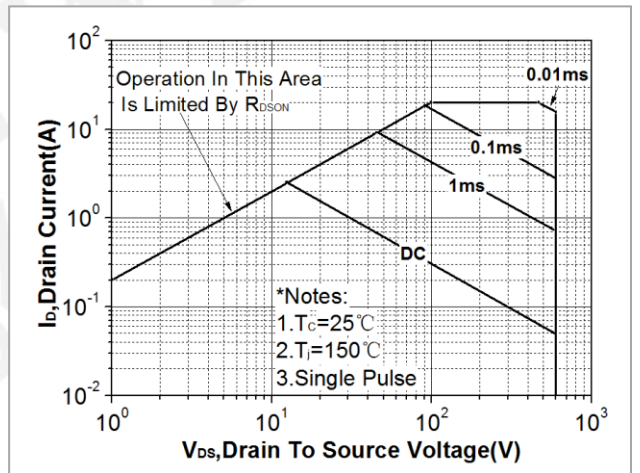
Fig. 10. Maximum safe operating area(TO-220SF)
