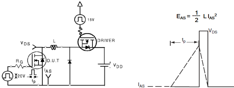
Fig. 16. Peak diode recovery dv/dt test circuit & waveform
