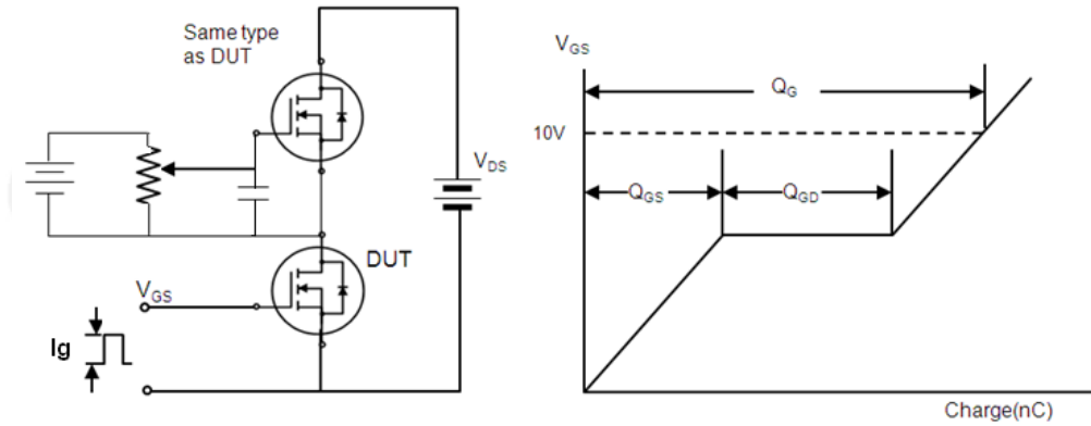
Fig. 16. Gate charge test circuit & waveform
