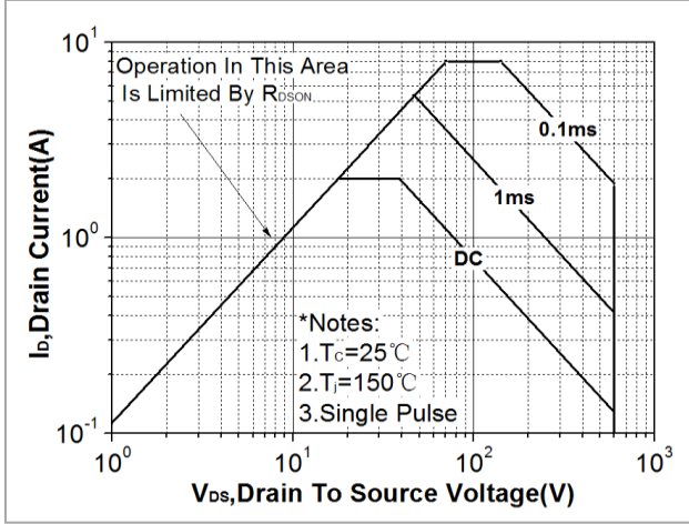
Fig. 7. Maximum safe operating area (TO-252&TO-251)
