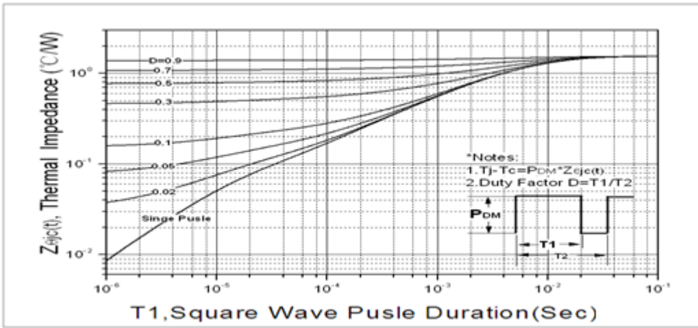
Fig. 9. Transient thermal response curve (TO-252&TO-251)
