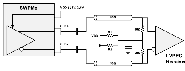
AC-Coupled Self-Biased LVEPCL - 50 Ω w/VTT Bias
