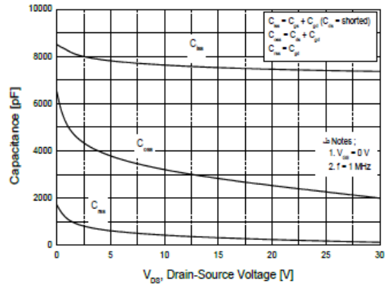
Fig.8 Capacitance Characteristics
